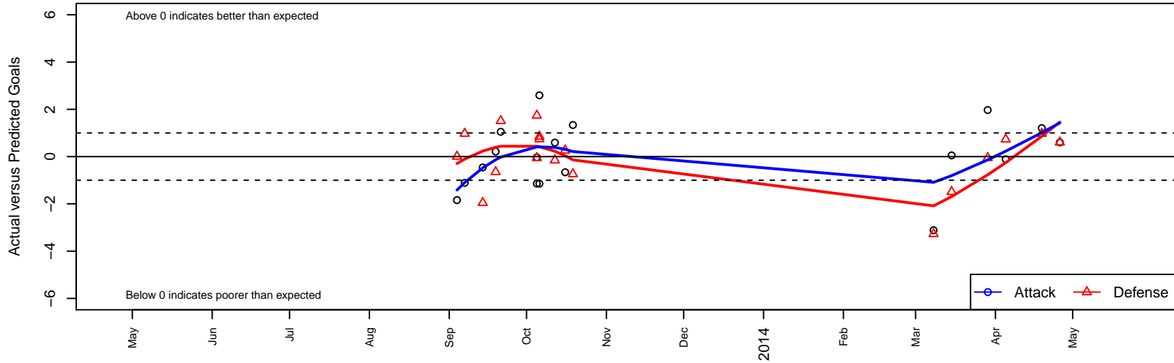
Idaho Rush Grey Dark G01 Dots are actual minus expected GF (blue circles) and GA (red triangles). Blue line is smoothed change in attack strength. Red is smoothed change in defense strength.
